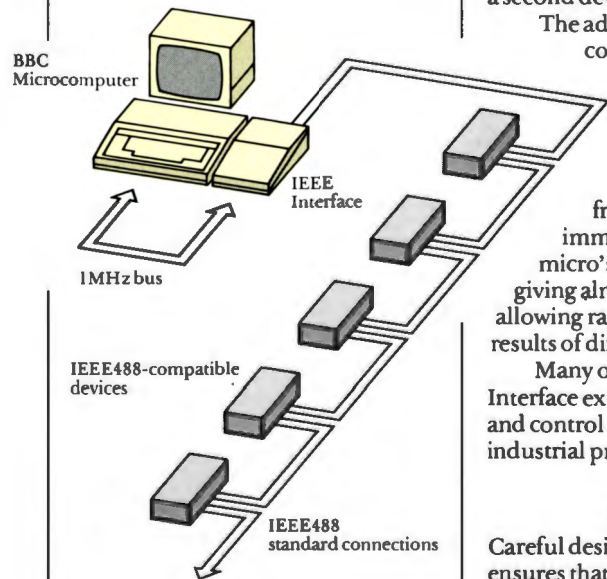
STRUCTURE OF AN IEEE NETWORK CONTROLLED BY A BBC MICROCOMPUTER
