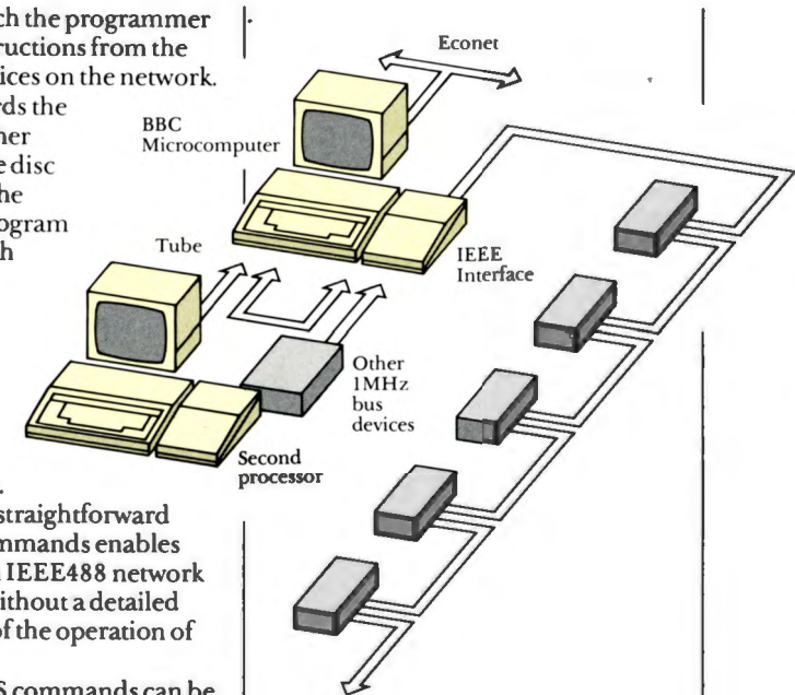
OTHER FACILITIES AVAILABLE WITH THE BBC MICROCOMPUTER/IEEE INTERFACE CONTROLLER
